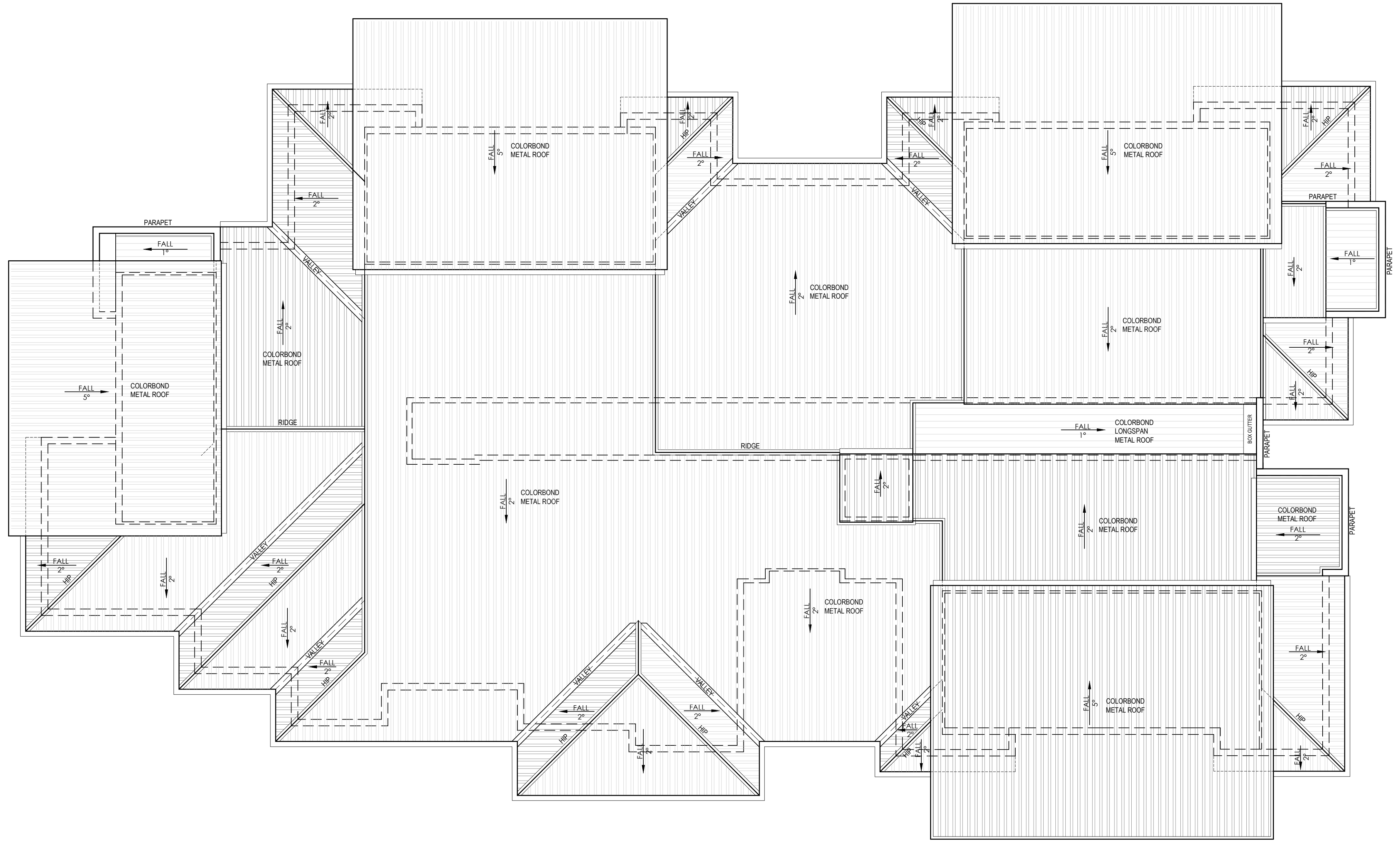
2 ILU BLOCK E - ROOF PLAN 1 : 100
